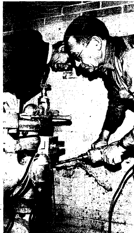
for injecting fluoride into a city water line before tapping the line so equipment can be installed.
